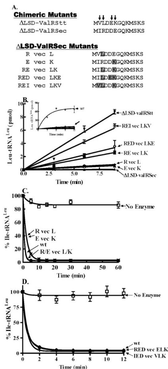
FIGURE 4: Enzymatic activity of derivatives of \Delta LSD-valRSec chimeric mutants. (A) Sequence of chimeric LeuRS mutants that contain a ValRS peptide insert and site-specific mutations within the inserted peptide of the \Delta LSD-valRSec chimeras. Sites that were targeted by specific substitution are indicated with arrows. Residues within the chimeric sequence \Delta LSD-valRSec that were substituted by the correlating T. thermophilus LeuRS residue are shaded. (B) Aminoacylation activity of chimeric mutants. The reaction was carried out using 4 \mu M in vitro transcribed tRNA Leu and 100 nM enzyme. An insert illustrates the wild-type activity relative to the mutants. The bold arrow within the insert identifies the region of the graph that has been blown up. (C) Post-transfer editing activity of single and double mutations of \Delta LSD-valRSec. (D) Post-transfer editing activity of triple mutations of \Delta LSD-valRSec. Post-transfer editing assays included about 6.5 \mu M [ 3 H]-Ile-tRNA Leu and 100 nM enzyme. Symbols representing wild-type and mutant enzymes are as follows: no enzyme ( \square ), wild type ( \circ ), \Delta LSD-valRStt ( \blacktriangledown ), \Delta LSD-valRSec ( \blacktriangle ), R vec L ( \blacklozenge ), E vec K ( \times ), RE vec LK ( * ), RED vec LKE ( \diamond ), and REI vec LKV ( + ). Error bars represent the assay reproduced at least in triplicate and are presented for each point.
