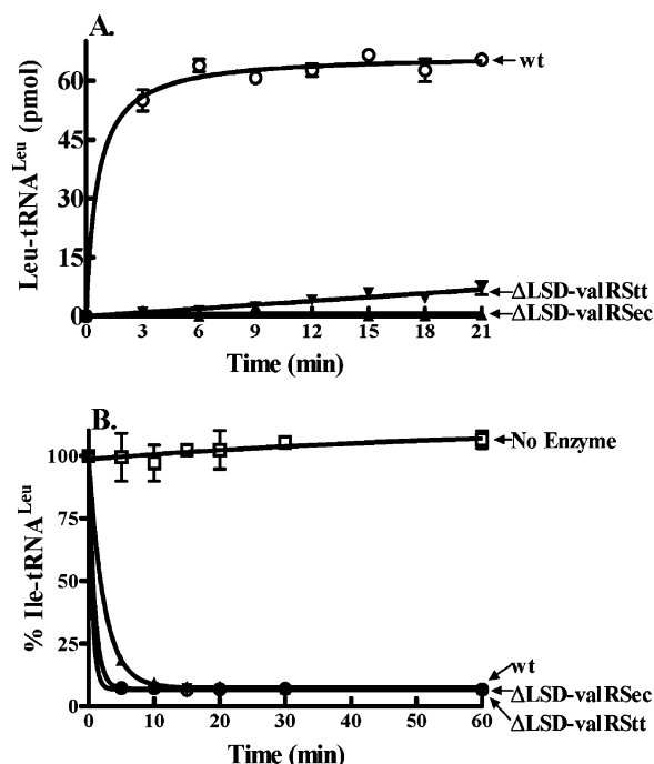
FIGURE 3: Enzymatic activity of chimeric LeuRS mutants. (A) Aminoacylation reactions were carried out using 4 \mu M in vitro transcribed tRNA Leu and 100 nM enzyme. (B) Post-transfer editing reactions included about 6.5 \mu M [ 3 H]-Ile-tRNA Leu and 100 nM enzyme. Symbols representing wild-type and mutant enzymes are as follows: no enzyme ( \square ), wild type ( \circ ), \Delta LSD-valRStt ( \blacktriangledown ), and \Delta LSD-valRSec ( \blacktriangle ). Error bars represent the assay reproduced at least in triplicate and are presented for each point.
