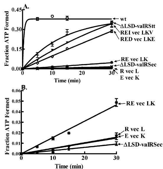
FIGURE 5: Pyrophosphate exchange activity of chimeric mutants. (A) The amino acid-dependent pyrophosphate exchange reaction was carried out in the presence of 1 mM leucine, 1 mM ATP, and 1 mM [\text{P}^{32}]\text{PP}_i . (B) Weakly active mutants in (A) are blown up. Symbols representing wild-type and mutant enzymes are as follows: wild type ( \circ ), \Delta\text{LSD-valRStt} ( \blacktriangledown ), \Delta\text{LSD-valRSec} ( \blacktriangle ), R vec L ( \blacklozenge ), E vec K ( \times ), RE vec LK ( * ), RED vec LKE ( \diamond ), and REI vec LKV ( + ). Error bars represent the assay reproduced at least in triplicate and are presented for each point.
